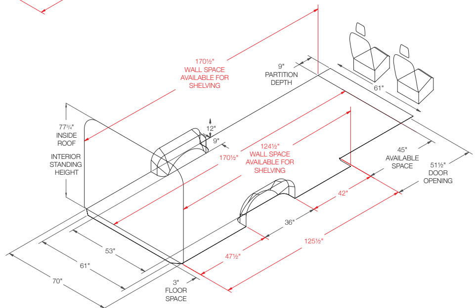
MERCEDES-BENZ SPRINTER 170" Extended Wheelbase
